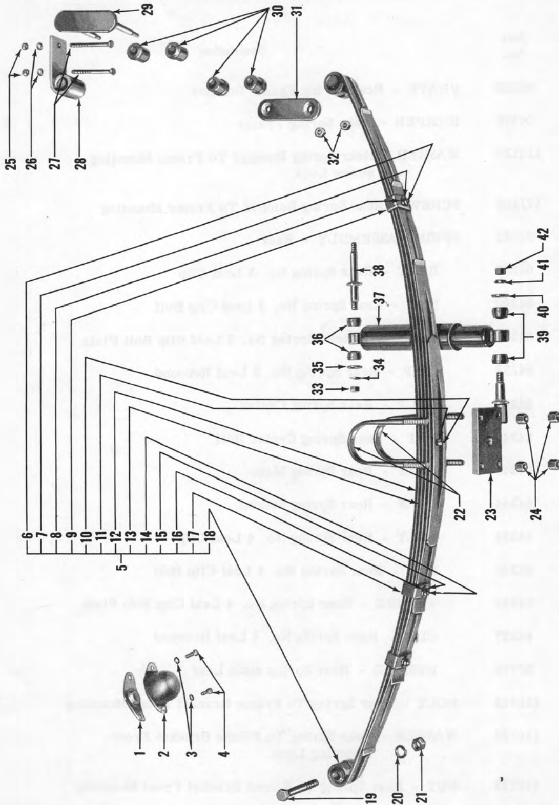
REAR SPRING and SHOCK ABSORBER INSTALLATION ILLUSTRATION No. 5
